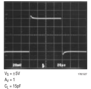
Small-Signal Response
